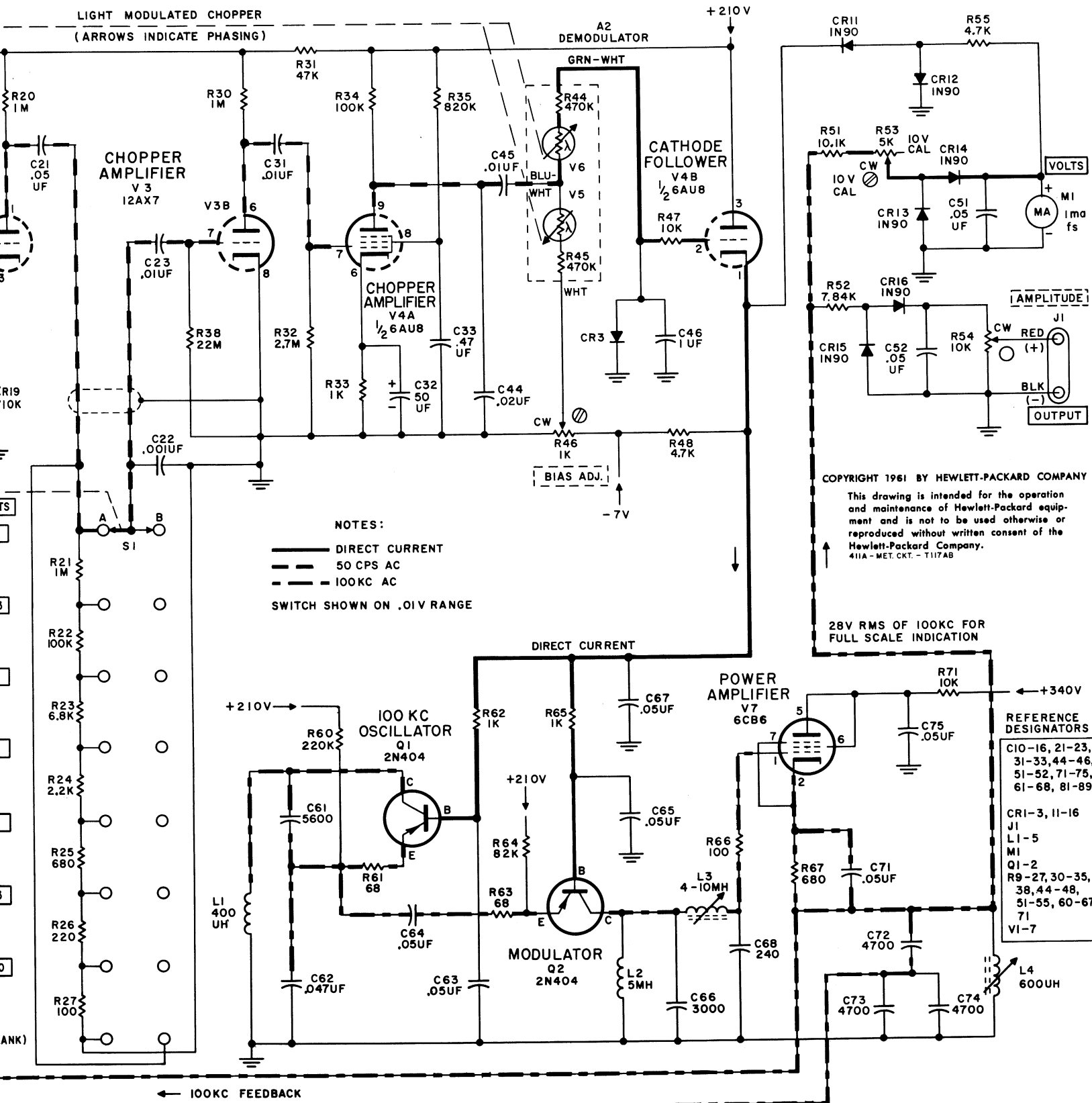
Figure 5-7. Voltmeter 5-11/5-1
